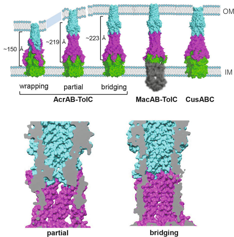
Fig. 2. Models for the tripartite drug efflux pumps. Three different complex models for the AcrAB-TolC pump (left three models), and the MacAB-TolC pump and CusABC pump, based on the adaptor bridging model. TolC or CusC are shown in cyan, the adaptor proteins (AcrA, MacA, and CusB) in magenta, and the inner membrane transporter (IMT; AcrB, MacB, and CusA) in green. Because of the lack of the full-length structure of MacB, the unknown transmembrane and cytosolic parts are shown in gray. There are also shown estimated distance (angstrom) between OM and IM spanned by each tripartite complex. Close-up views of the vertical sections of the AcrA-TolC assembly based on the adaptor partial wrapping model and the adaptor bridging model are shown at the bottom.
